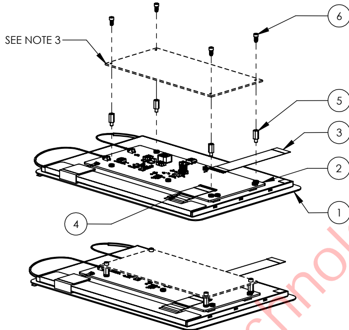
PHYTEC BOARD MOUNTING
