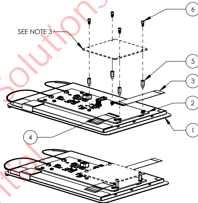
BEAGLE BOARD MOUNTING
